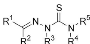
Figure 1. General structure of TSC. R1, R2, R3, R4, R5 = H, or an organic substituent.
